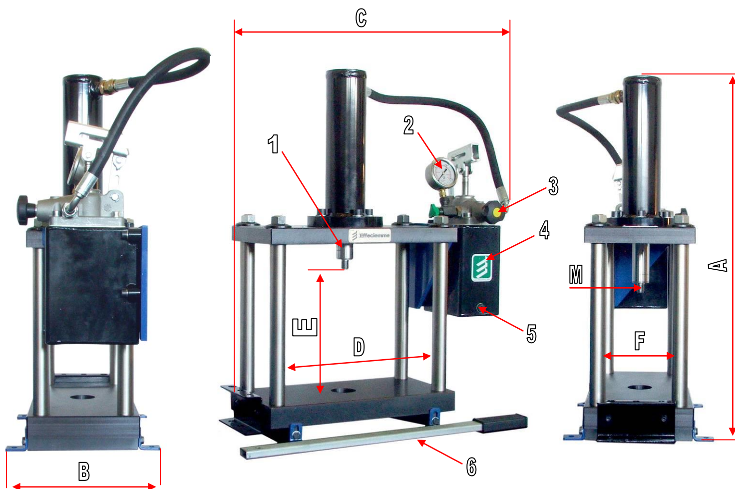
HYDRAULIC PRESS Art. PR-10T – 10 Ton.
