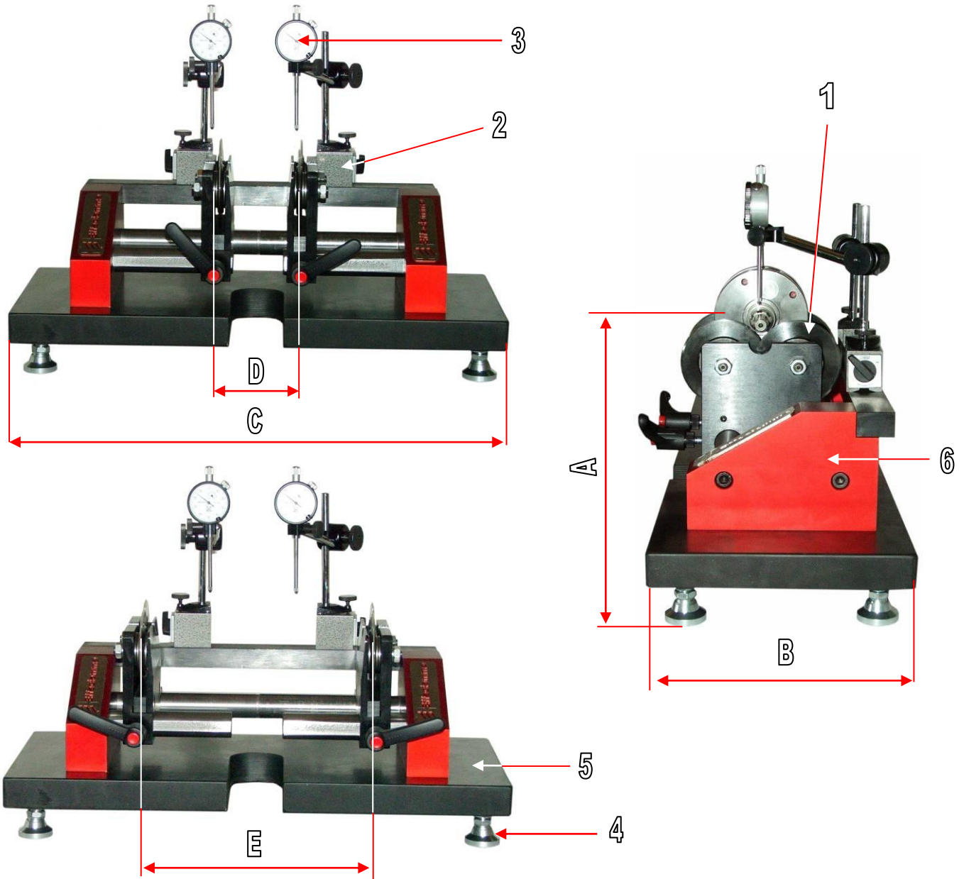
BALANCING BENCH FOR CRANKSHAFTS - Art. BEA275
